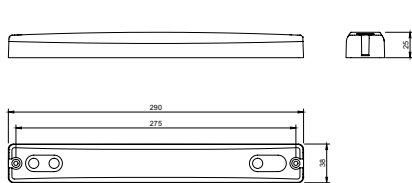
HANGING KIT
