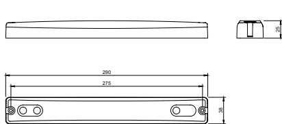
HANGING KIT
