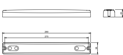
HANGING KIT
