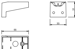
SIDE MOUNT KIT
