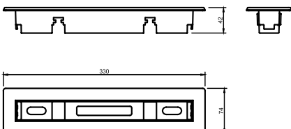
RECESSED KIT
